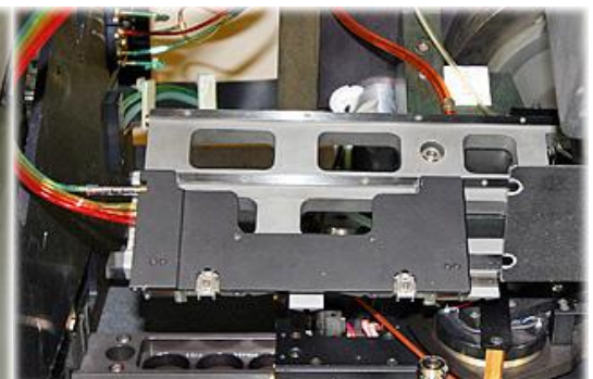
1500 Reticle Stage
